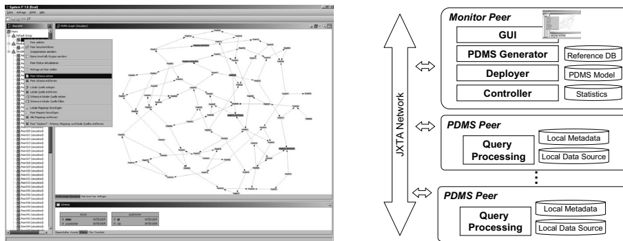
Figure 1: Screenshot of the monitor peer of System P with automatically generated PDMS (left) and architecture of System P with monitor peer and PDMS peer (right).
